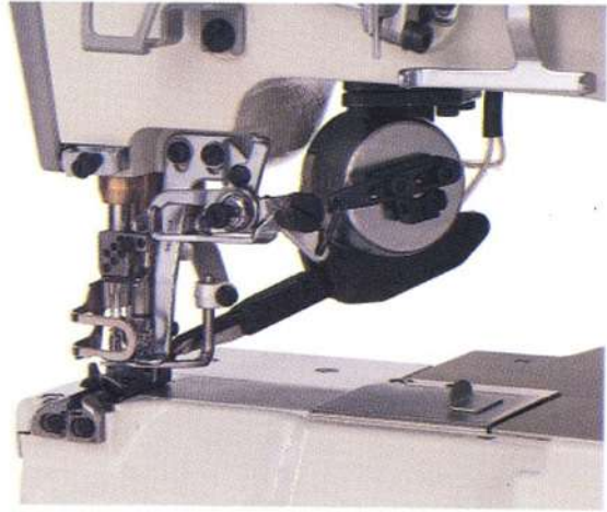
Top and underbed thread trimmer (Electric)
