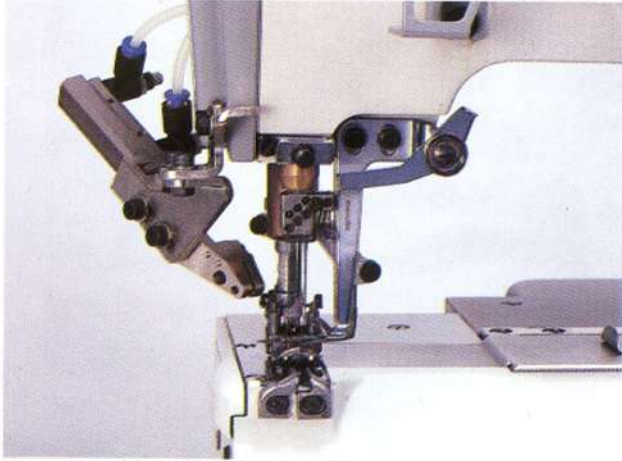
Top and underbed thread trimmer (Pneumatic)
